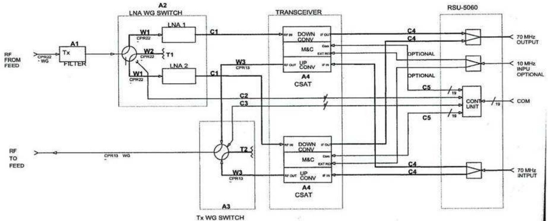
Figure B-1. Typical CSAT Redundant System
