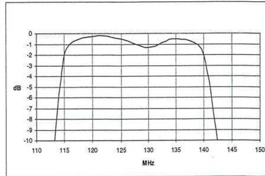
Figure D, Typical passband response, RF bandpass input filter.
