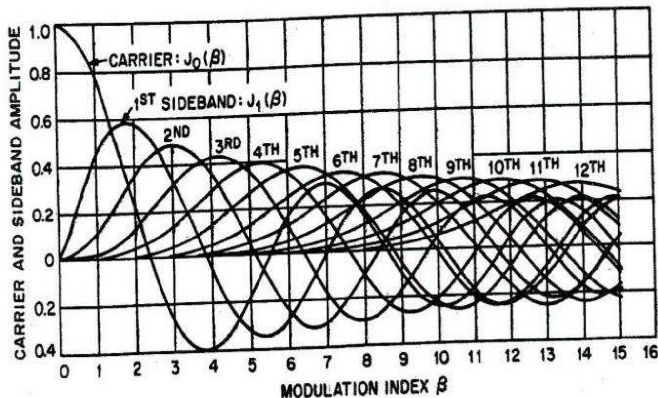
Fig. 17—Plot of Bessel functions of first kind as a function of argument \beta . From P. F. Panter, "Modulation, Noise, and Spectral Analysis," Fig. 7-8, © 1965, McGraw-Hill Book Company.
