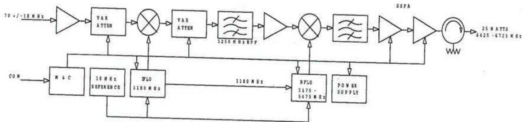
Figure D-2. Functional Block Diagram of the Upconverter Section
