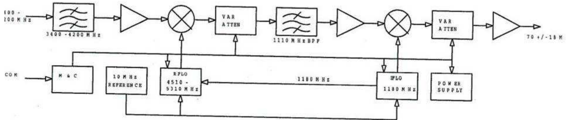
Figure D-1 Functional block diagram of the downconverter section
