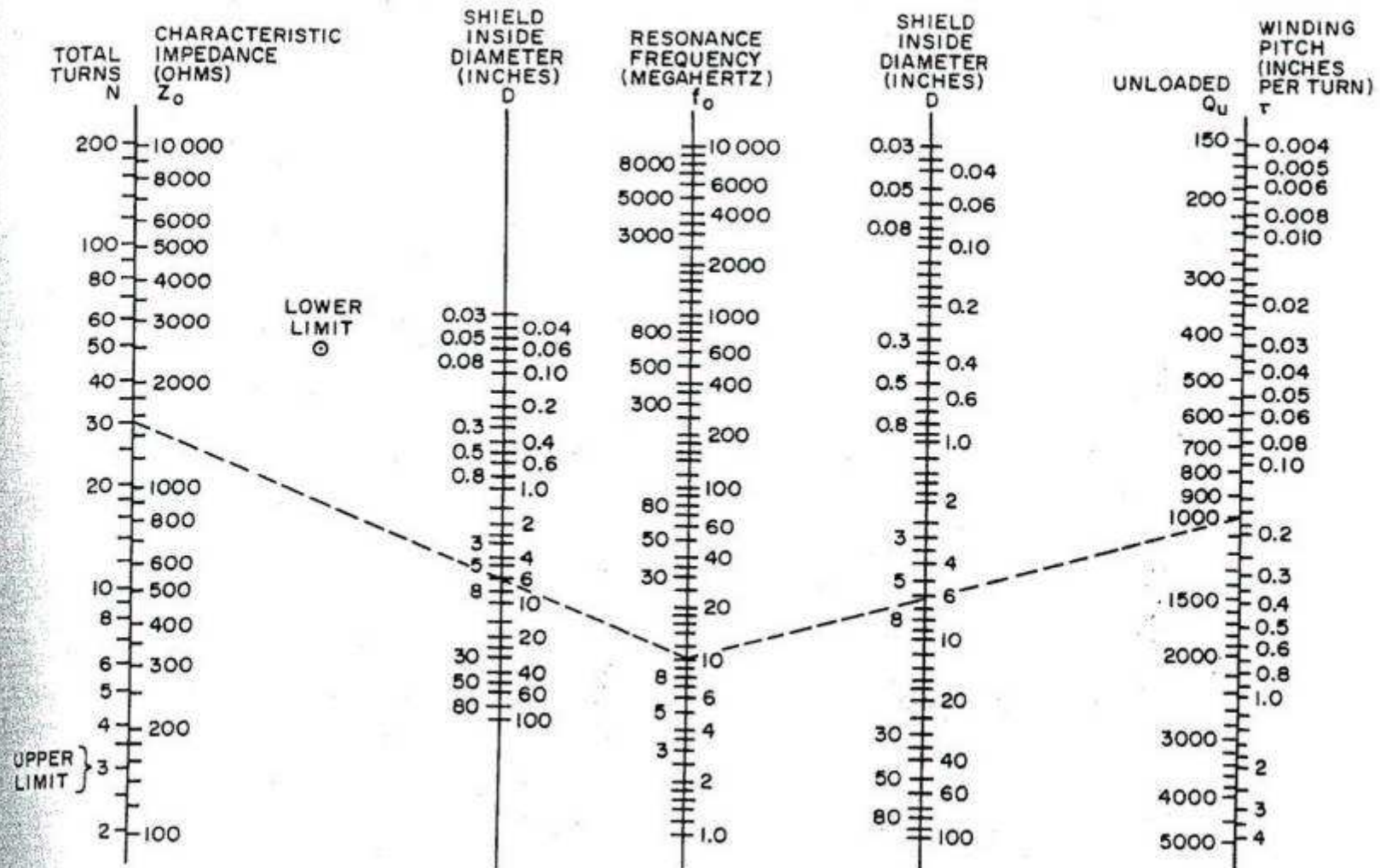
Fig. 34—Design chart for quarter-wave helical resonators. W. W. Macalpine and R. O. Schildknecht, "Coaxial Resonators with Helical Inner Conductor." Proceedings of the IRE , vol. 47, no. 12, p. 2101, December 1959. © 1959
