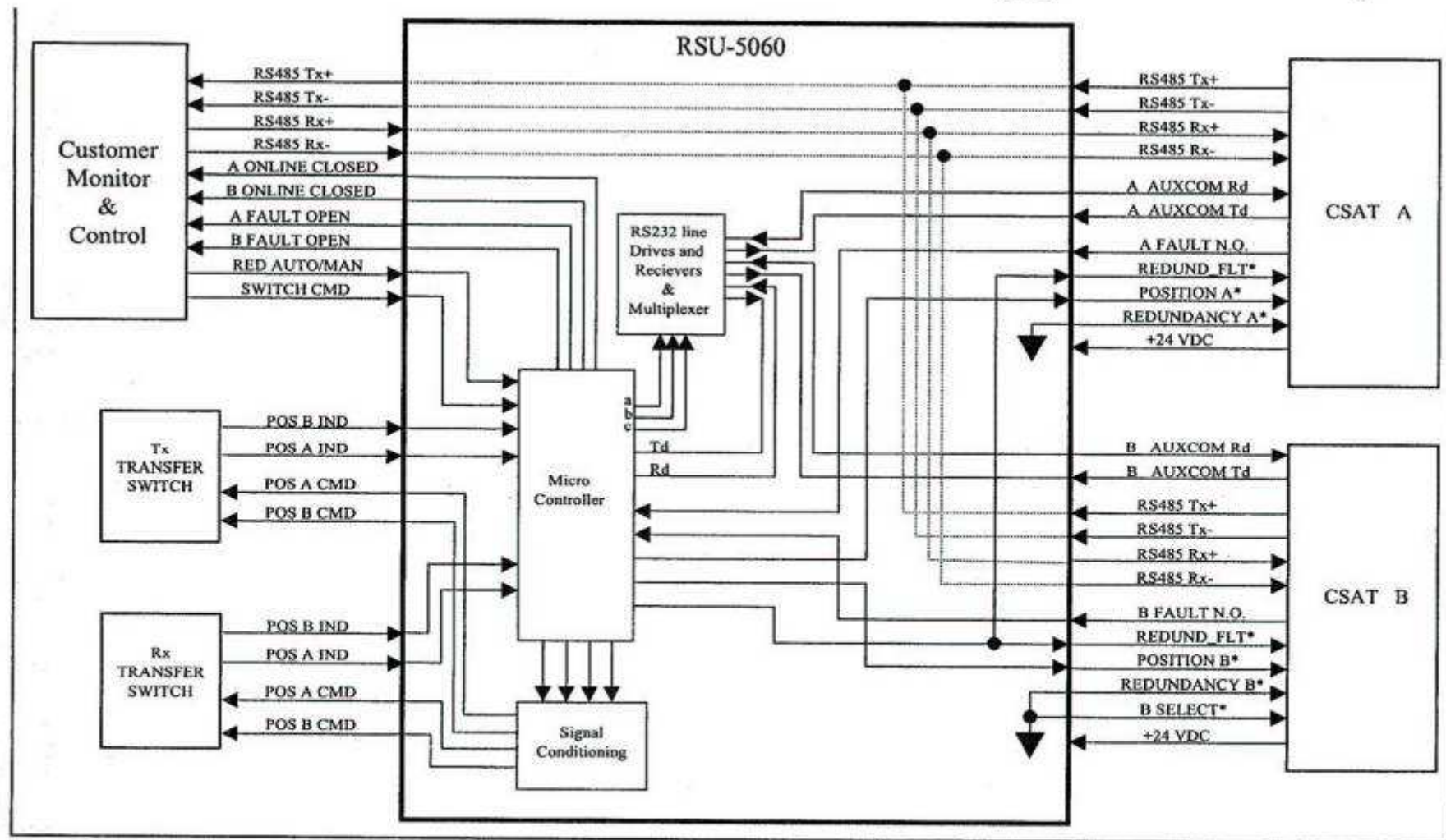
Figure B-3 RSU-5060 Functional Block Diagram
