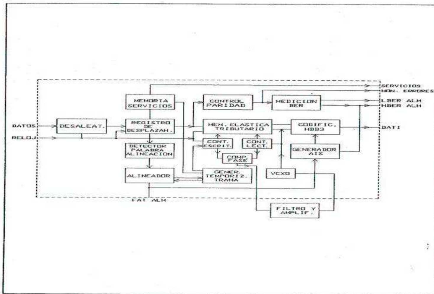
Fig. 8 - Gate Array Bit Extraction
