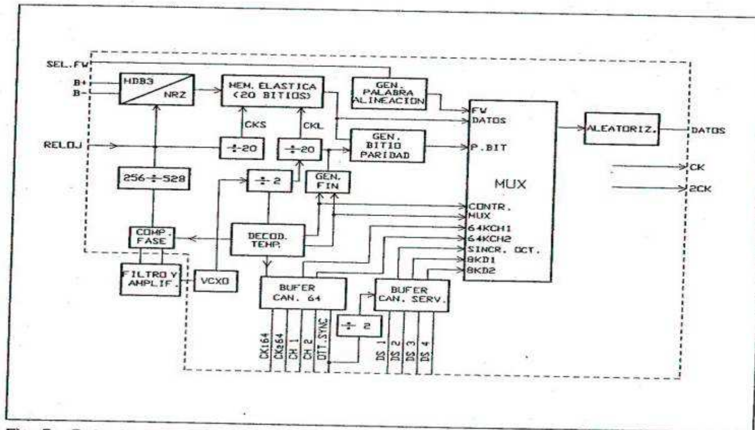
Fig. 5 - Gate Array Bit Insertion
