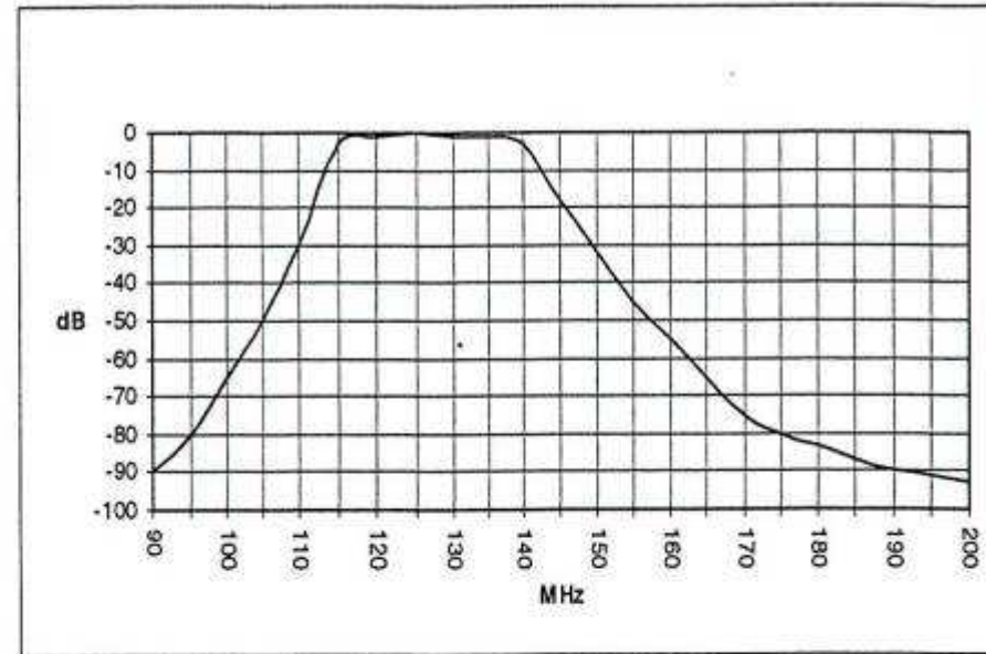
Figure C, Typical response, RF bandpass input filter.
