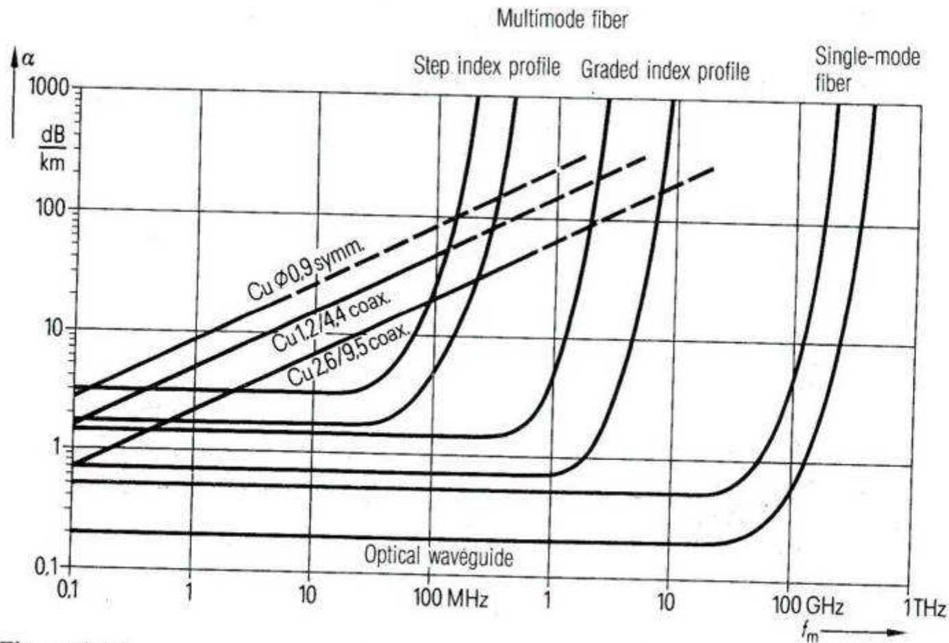
Figure 9.12 Attenuation coefficient as a function of the frequency of modulation for balanced and coaxial copper cables and for various optical cables
