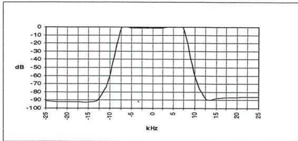
Figure F, Typical 455 kHz IF response (25 kHz channels)
