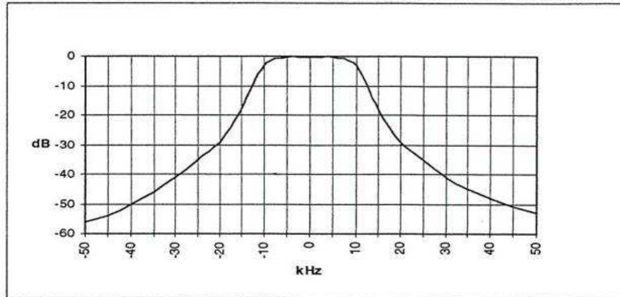
Figure E, Typical 45 MHz IF response
