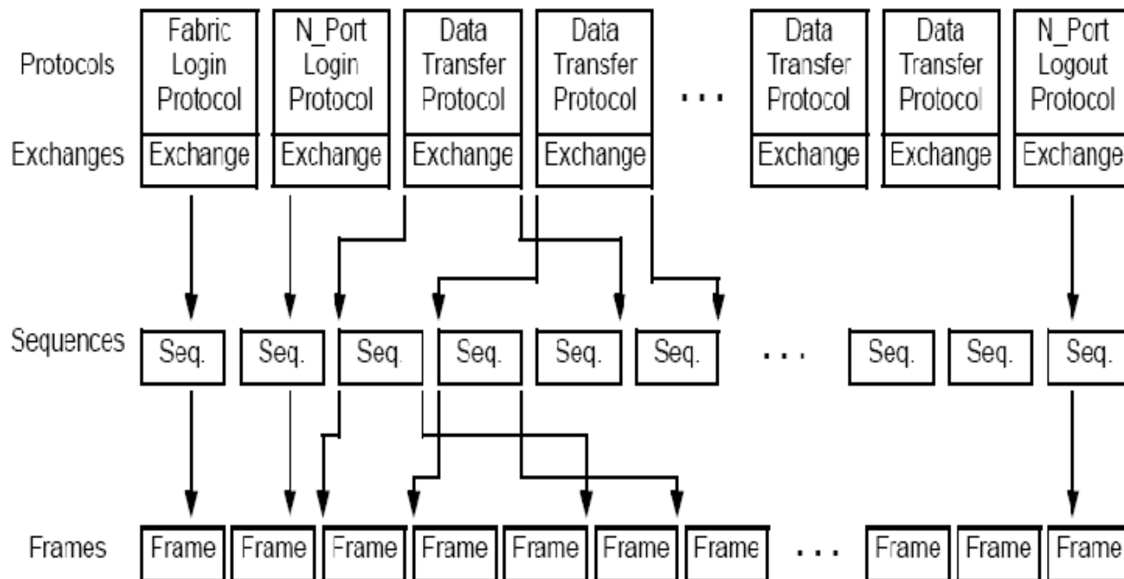
Figure 8 - FC-2 building block hierarchy
